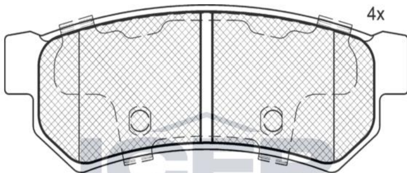
Loose Shim
